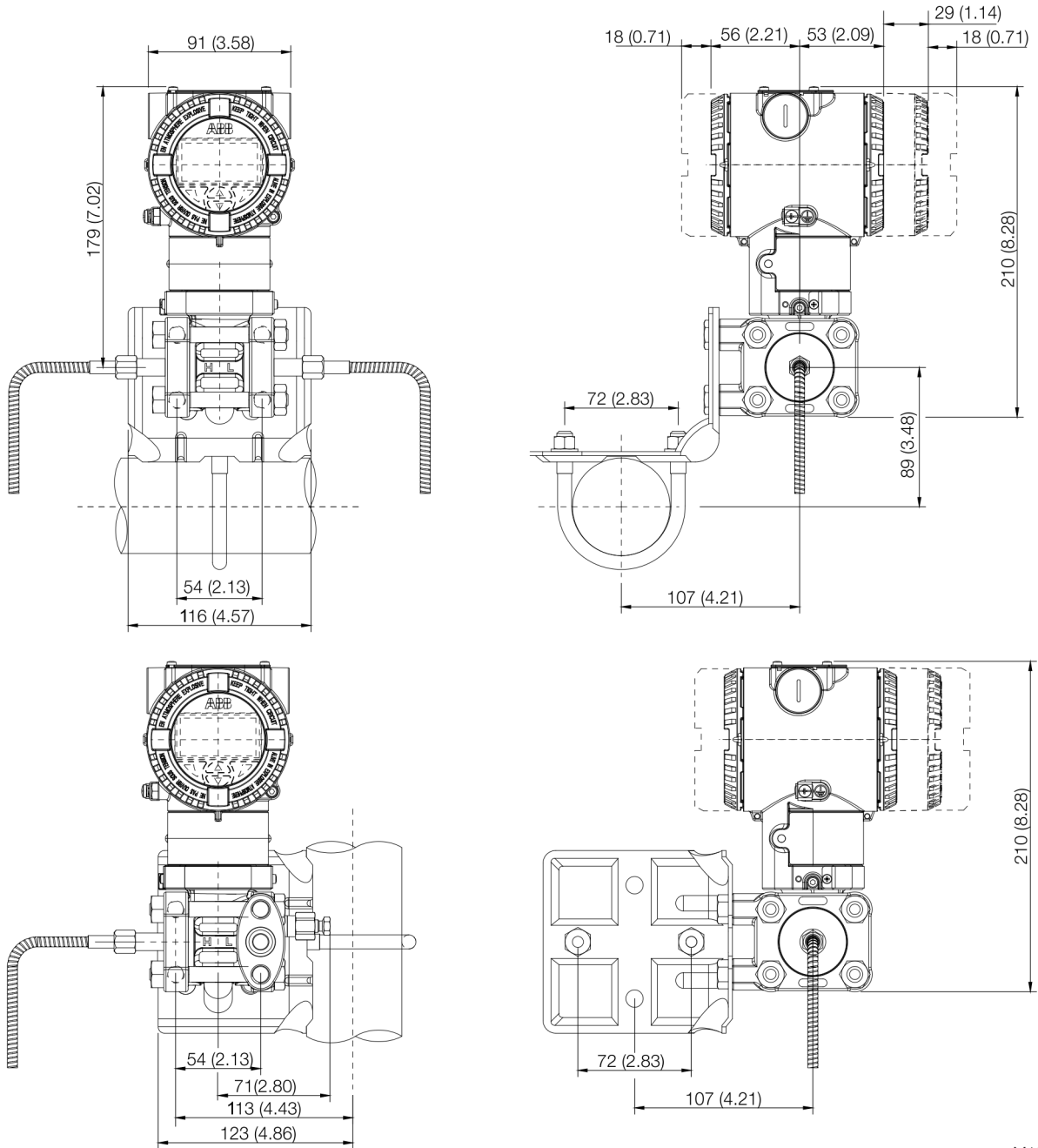
Figure 6: Pipe mounting - Barrel housing
